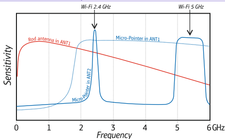
Sensitivity graph of the Protect 1206i
